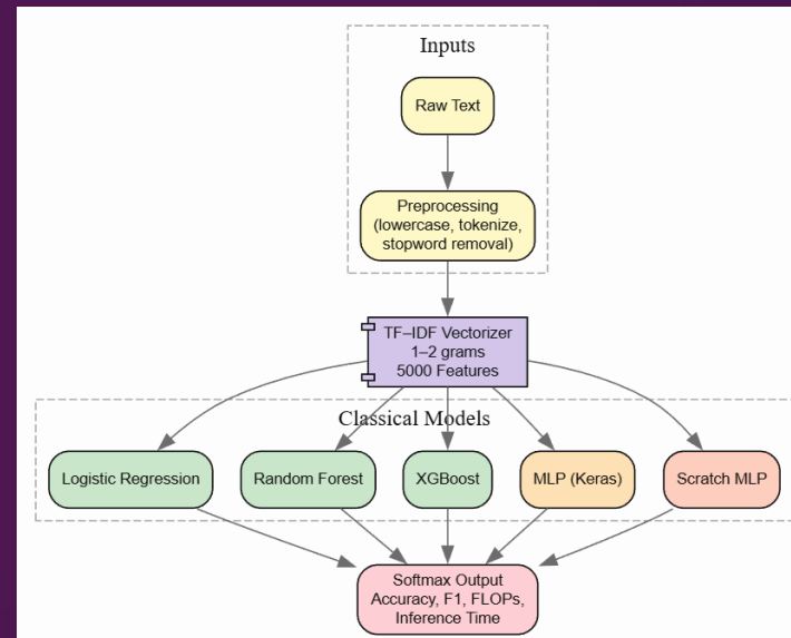
Figure: TF-IDF Vectorizer Workflow for different Models
