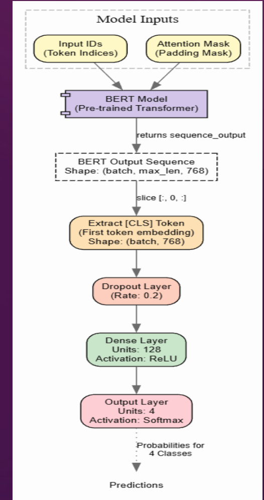
Figure: BERT with an MLP Classification Layer Models
