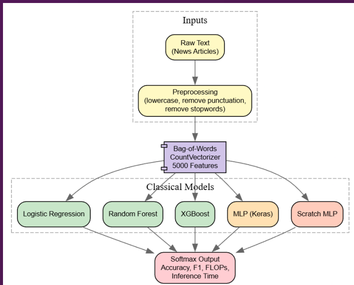
Figure: Bag of Words Vectorizer Workflow for different Models
