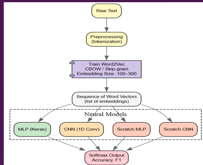
Figure: Word2Vec with Neural Network Models
